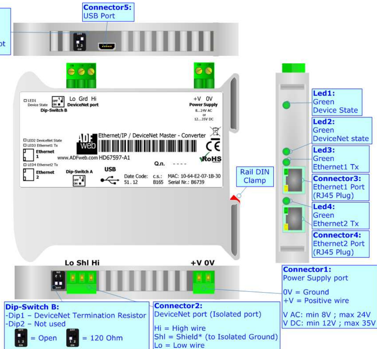
Figure 1: Connection scheme
