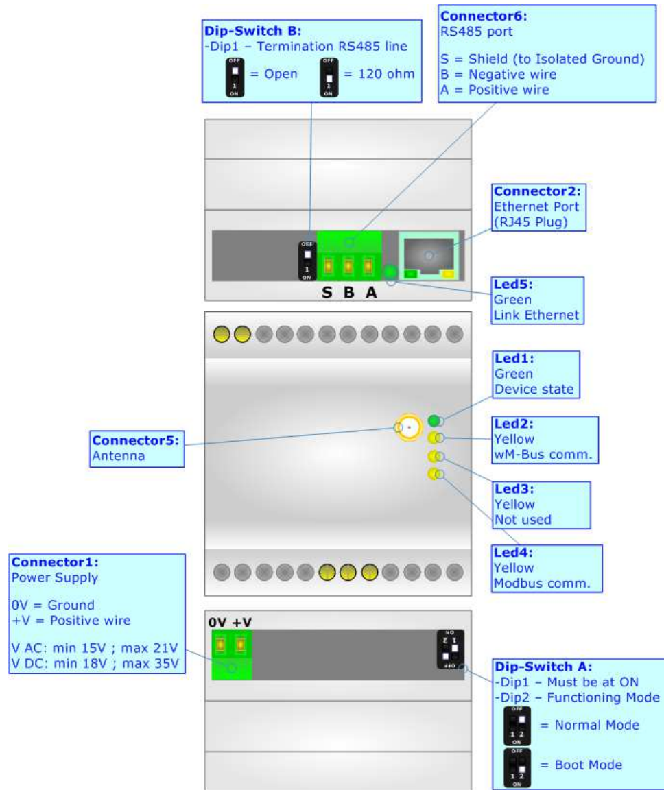
Figure 1a: Connection scheme
