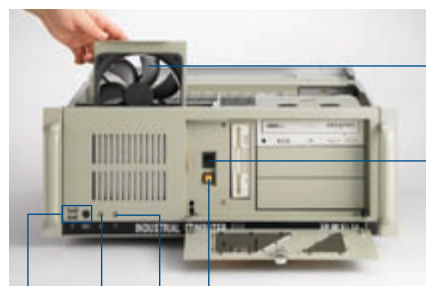
HDD LED Power button USB & PS/2 Power LED
