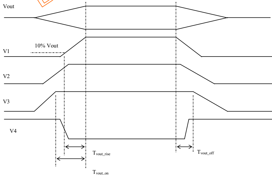
Figure 2: Power Supply Timing
