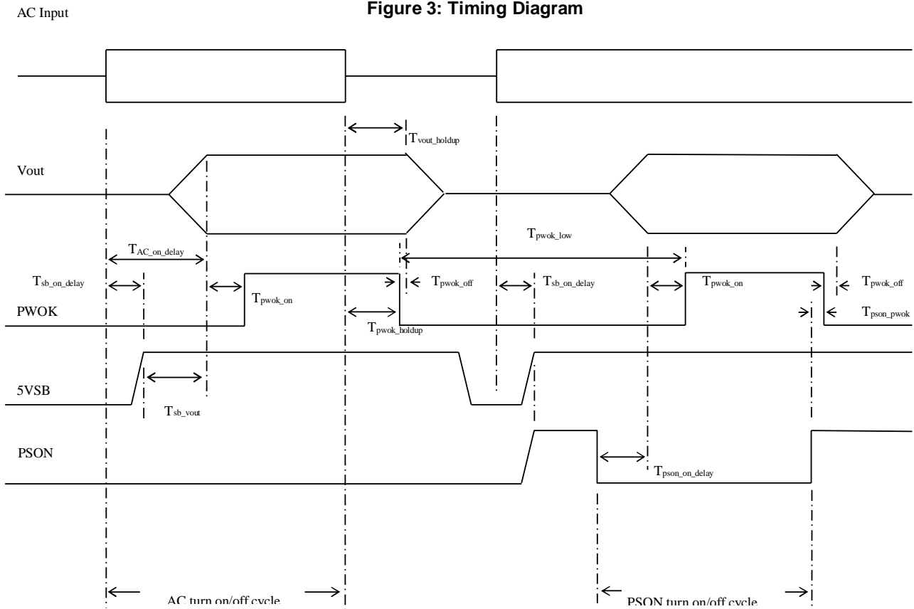
Figure 3: Timing Diagram
