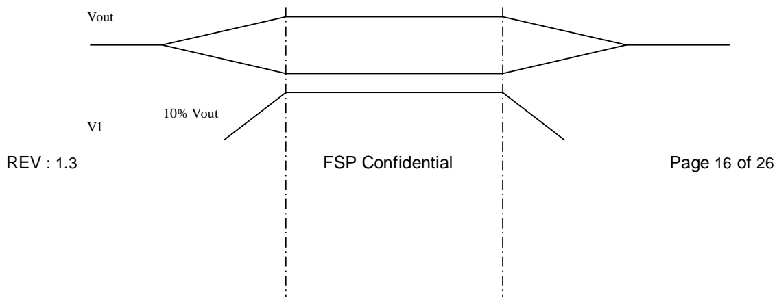
Figure 2: Power Supply Timing
